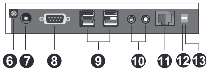
CE924R (Remote Unit) Rear View
