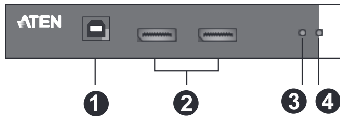
CE924L (Remote Unit) Rear View
