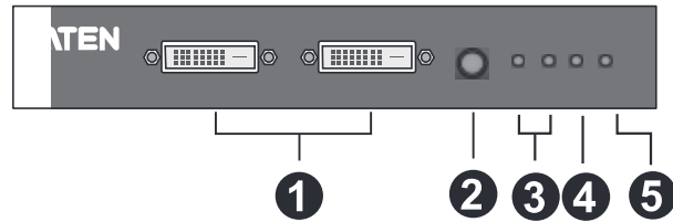
CE624R (Remote Unit) Rear View
